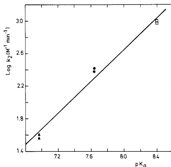
Figure 1. Log k 2 (M -1 min -1 ) vs. pK a for the reactions of 1 (●), 2 (□), and 3 (▲) with sarin in aqueous solution at 25 °C.
