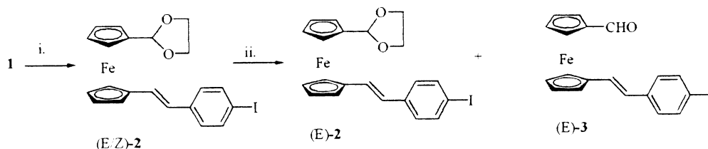
Scheme 2. (i) p -Iodobenzyltriphenylphosphonium bromide; \text{KO}^t\text{Bu} ; (ii) \text{I}_2 , sunlight.
