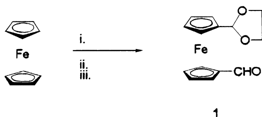
Scheme 1. (i) BuLi, hexane, TMEDA, diethyl ether; (ii) DMF, -78^{\circ}\text{C} ; (iii) (\text{HOCH}_2)_2 , \text{H}^+ .
