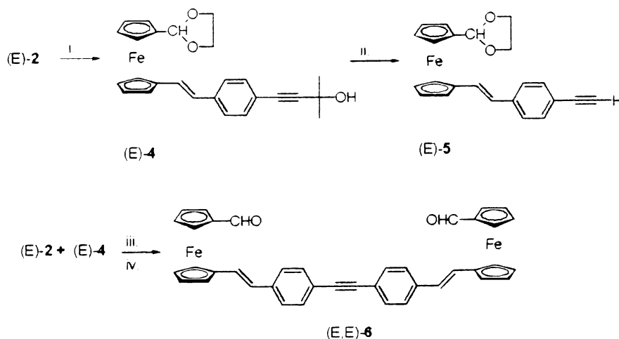
Scheme 3. (i) \text{PdCl}_2(\text{PPh}_3)_2 , \text{Cu}_2\text{I}_2 , \text{NEt}_3 , \text{HC}\equiv\text{C}(\text{CH}_3)_2\text{-OH} ; (ii) \text{NaOH} , toluene, \Delta ; (iii) \text{PdCl}_2(\text{PPh}_3)_2 , \text{Cu}_2\text{I}_2 , \text{NEt}_3 ; (iv) \text{AcOH} , \text{H}_2\text{O} .
