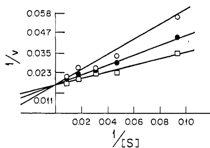
Figure 1. Double reciprocal plot for galactosyltransferase activity in the presence of uridine 5'-[( \alpha -D-galactopyranosylhydroxyphosphinyl)methyl]phosphonate (O, 33 \mu M; \bullet , 17 \mu M; \square , 10 \mu M; \triangle , 0 \mu M). Enzyme activity was measured as described in the Experimental Section. UDP-galactose concentrations were varied from 1 to 80 \mu M.
