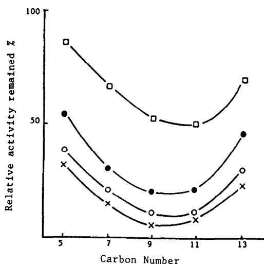
Fig. 2. Effect of the length of alkyl side chain of bromoquinone derivatives on ubiquinol cytochrome c reductase activity. (●) I, (x) II, (○) III and (◻) IV. The mola ratio of bromoquinones to cytochrome c 1 (succinate cytochrome c reductase) was set at 6:1. The experimental conditions and other symbols are the same as the legend of Fig. 1.
