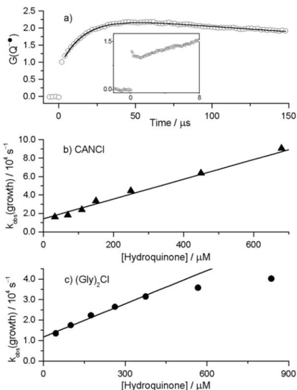
Fig. 5 Graphs showing the data obtained following pulse radiolysis of chloramines/amides in the presence of the readily oxidised quencher, QH 2 : a) a kinetic trace ( \lambda , 427 nm; [CANCl], 310 \mu\text{M} ; [QH 2 ], 450 \mu\text{M} ; 10% tert -butyl alcohol) showing a rapid absorption increase due to \text{e}^-_{\text{aq}} absorption, followed by growth and decay of Q•. Raw data are shown as open circles, with the calculated fit shown by a solid line. Inset shows the absorbance changes occurring due to \text{e}^-_{\text{aq}} decay and Q• formation in the first 8 \mu\text{s} following the pulse. Absorbance is given in terms of G , which represents the approximate micromolar concentration per 10 J absorbed energy. b) Plot showing the pseudo-first order rate of formation of Q• following pulse radiolysis of 10% tert -butyl alcohol solutions (under N 2 ) containing 310 \mu\text{M} CANCl in the presence of increasing [QH 2 ]. c) Plot showing the pseudo-first order rate of formation of Q• following pulse radiolysis of 10% tert -butyl alcohol solutions (under N 2 ) containing 300 \mu\text{M} (Gly) 2 Cl in the presence of increasing [QH 2 ]. Linear fit provides a maximal estimate of the second-order rate constant for radical quenching by QH 2 .
