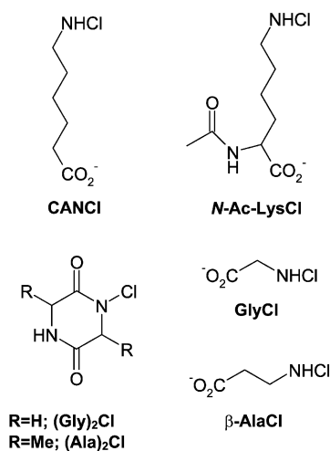
Scheme 1 Structures of the chloramines/amides used in these studies: 6-aminohexanoic acid chloramine, CANCl; \alpha - N -acetyl-Lys chloramine, N -Ac-LysCl; Gly chloramine, GlyCl; \beta -Ala chloramine, \beta -AlaCl; cyclo-(Gly) 2 chloramide, (Gly) 2 Cl; cyclo-(Ala) 2 chloramide, (Ala) 2 Cl.
