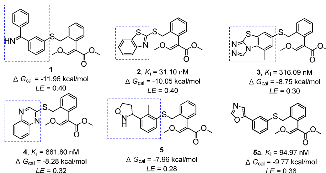
Figure 2. Chemical structures of five final candidates. The fragments determined by PFVS are shown in blue boxes. 5a is a synthetic analogue of compound 5 . Ligand efficiency (LE) value is defined as the calculated binding free energy ( \Delta G_{\text{cal}} ) divided by the HAC, LE = -\Delta G_{\text{cal}}/\text{HAC} .
