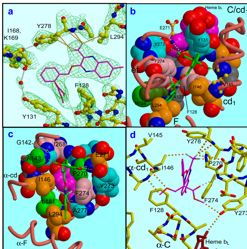
Figure 7. X-ray structure of 4e bound to chicken bc_1 complex. Residues are numbered according to the bovine/swine sequence. (a) Overall shape of the inhibitor and quality of the electron density (2Fo-Fc map contoured at 1.5 \sigma ). Multiple van der Waals contacts of the trifluoromethyl group with residues 278 and 294 are shown as brown and H-bonds between the residues as white, dotted lines. (b) Space-filling model of the "bottom" of the binding pocket, viewed from above. The inhibitor is shown as a stick figure with green carbons. The pharmacophore, at right angles to the rest of the molecule, fits into a slot at upper right and contacts Glu271, Phe274, and Ala143. The side-chain quinoxaline ring stacks with Phe274. (c) Stick figure model, detailing interactions of the pharmacophore and trifluoromethyl group with the protein. Distances are described in Table 2, Supporting Information. Stereo views of these figures are available in Figure 6, Supporting Information. (d) Space-filling model of the top of the binding pocket, viewed from below. Tyr278 (magenta, unlabeled) blocks the hole in the "top" through which the ISP accesses the site. The phenyl "bridging" ring of the inhibitor inserts between Pro270 and the cd_1 helix at 142–243. The trifluoromethyl group protrudes between Ile146, Phe274, Ala277, and Leu294. Dotted lines show the C-F...H interactions. Both the trifluoromethyl group and the bridging ring make multiple contacts with Tyr278. Stacking of the quinoxaline ring with Phe274 and contacts of the pharmacophore with Glu270, Tyr273, and the cd_1 helix can also be seen.
