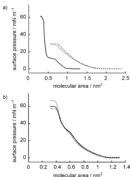
Figure 2. \pi - A Isotherms of a) 1 and b) 2 on aqueous \text{H}_2\text{SO}_4 (pH 2, —), pure water (pH 6, ----) and aqueous \text{NH}_4\text{OH} (pH 12, .....), at 20°C.
