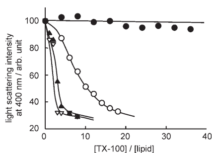
Figure 5. Light scattering intensities of the cerasomes prepared from 1 or 2 , and DMPC-liposome as a function of added equivalents of TX-100 at 25°C: cerasome of 1 incubated for 24 h (●); cerasome as-prepared from 1 (○); cerasome of 2 incubated for 24 h (▲); DMPC-liposome (▽).
