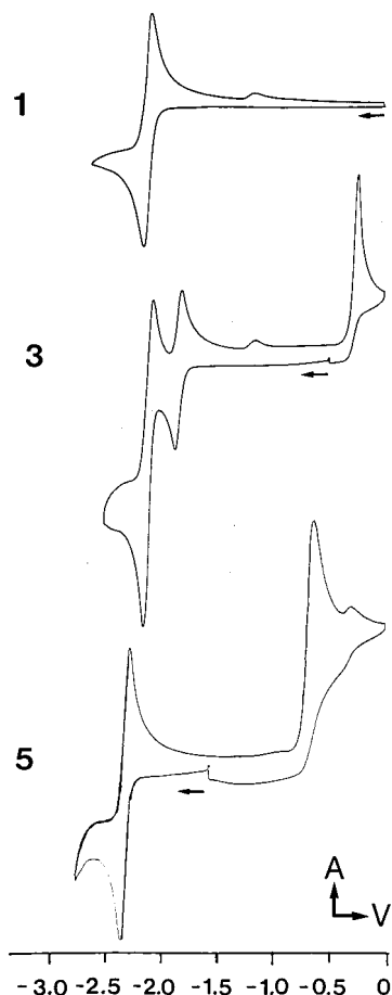
Figure 3. Cyclic voltammograms for arsenine (1), bis(arsenine)titanium (3), and bis(benzene)titanium (5) in DME/ n -Bu 4 NClO 4 at -45^\circ\text{C} vs SCE (100 mV/s).
