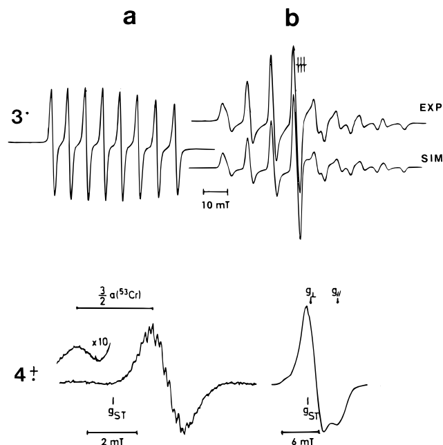
Figure 4. EPR spectra (X-band) of the (\eta^6\text{-arsenine})\text{metal} ( d^5 ) species \mathbf{3}^+ ( \text{M} = \text{V} ) and \mathbf{4}^{+} ( \text{M} = \text{Cr} ) in fluid (a) and rigid (b) solution (ST = Frémy salt, \langle g \rangle = 2.0057 ). \mathbf{3}^+ (toluene, 300–120 K): \langle g \rangle = 1.9897 , g_z = 2.002 , g_x = 1.9906 , g_y = 1.9765 , a(^{51}\text{V}) = -7.34 , A_z = -2.06 , A_x = -9.29 , A_y = -10.65 mT, a(^1\text{H}) = 0.31 mT. \mathbf{4}^{+} (DMF/ \text{CHCl}_3 (1:1), 298–140 K): \langle g \rangle = 1.9895 , g_{\parallel} = 1.9730 , g_{\perp} = 1.9977 , a(^{53}\text{Cr}) = 1.93 mT. The superhyperfine structure defies analysis.
