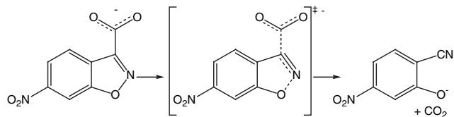
Scheme 1. Decarboxylation reaction of 6-nitrobenzisoxazole-3-carboxylate (6-NBIC)
