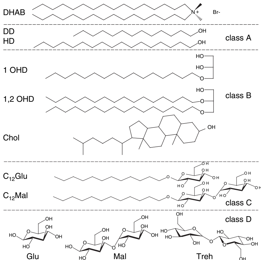
Scheme 2. Structure of DHAB (top) and the four classes of additives A–D: (A) DD is n -dodecanol and HD is n -hexadecanol; (B) 1-OHD is 1- O - n -hexadecyl-rac-glycerol, 1,2-OHD is 1,2- O -di- n -hexadecyl-rac-glycerol and Chol is cholesterol; (C) C_{12} Glu is n -dodecyl- \beta -D-glucopyranoside, and C_{12} Mal is n -dodecyl- \beta -maltoside; (D) Glu is glucose, Mal is maltose and Treh is trehalose
