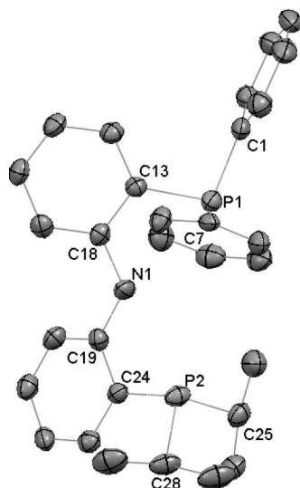
Figure 1. Molecular structure of H[Ph-PNP- i Pr] ( 1d ) with thermal ellipsoids drawn at the 35% probability level.
