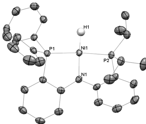
Figure 4. Molecular structure of [\text{Ph-PNP-}i\text{Pr}]\text{NiH} ( 2d ) with thermal ellipsoids drawn at the 35% probability level.
