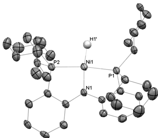
Figure 3. Molecular structure of [\text{Cy-PNP}]\text{NiH} ( 2c ) with thermal ellipsoids drawn at the 35% probability level.
