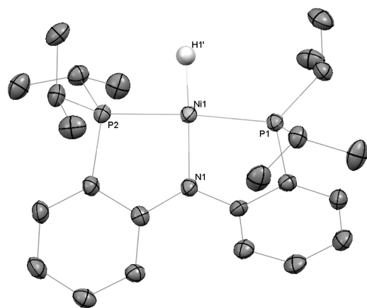
Figure 2. Molecular structure of [i\text{Pr-PNP}]\text{NiH} ( 2b ) with thermal ellipsoids drawn at the 35% probability level.
