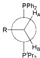
Figure 6. Newman projection of [\text{Ph-PNP-}i\text{Pr}]\text{NiCH}_2\text{R} ( \text{R} = \text{Me} ( 4d ), n -pentyl ( 5d )) along the \text{Ni-C}_\alpha bond.
