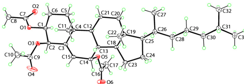
Fig. 2. Molecular structure of 4aa and atom labelling.
