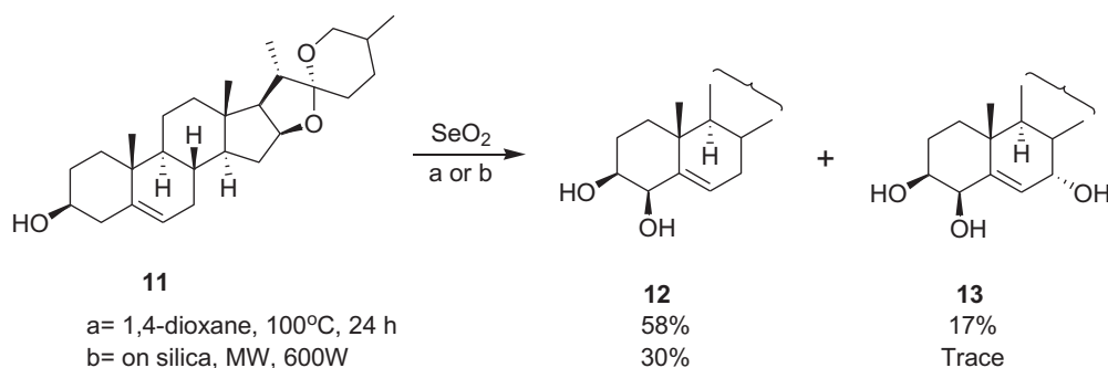
Scheme 4. Action of SeO 2 on diosgenin ( 11 ).
