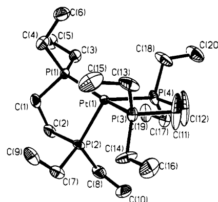
Figure 1. Perspective view of the molecular configuration of Pt(depe) 2 H + (3) with the atom-numbering scheme for non-hydrogen atoms. The thermal ellipsoids are scaled to enclose 50% probability.
