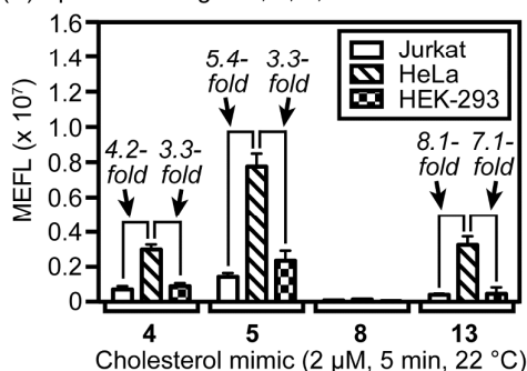
Fig. 3. Total binding (A) and specific binding (B) of compounds 4 , 5 , 8 , and 13 to three mammalian cell lines. Cells in media containing 10% serum were treated with compounds, without (A) and with (B) excess ezetimibe ( 3 , 200 \mu M), in triplicate at 22 ^{\circ} C for 5 min. Jurkat, HeLa, and HEK-293 cells were suspended in media prior to treatment and analysis of fluorescence by flow cytometry.
