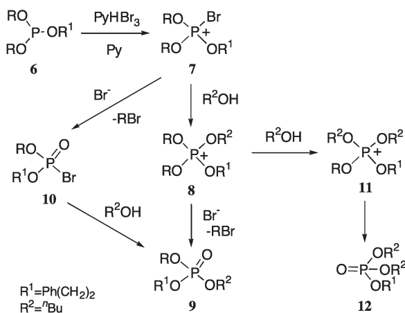
Scheme 1. Mechanistic pathways.
