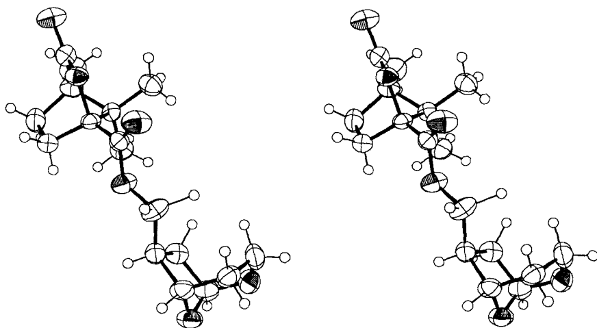
Figure. Stereoscopic view of 14 . Vibrational ellipsoids are drawn at the 50% level using ORTEP [18]. Orthorhombic space group P2_12_12 , Z = 4 with cell dimensions a = 6.185(2) , b = 13.345(5) , c = 21.812(9) Å. Intensities were measured at room temperature with an Enraf Nonius CAD4 diffractometer equipped with a graphite monochromator ( \text{MoK}_\alpha , \lambda = 0.7107 Å). Of the 1693 independent reflections ( \theta < 25^\circ ), 824 with I > 3\sigma(I) were used in the refinement. The structure was solved by direct methods with SHELXS-86 [19], and refined by full-matrix least-squares analysis [20]. Non-H-atoms were refined anisotropically. The positions of the H-atoms were calculated and refined isotropically in the final least-squares cycles. The weighting scheme used was \sigma(F)^{-2} . The refinement converged at R = 0.032 , R_w = 0.038 . Atomic positional and anisotropic displacement parameters for the non-H-atoms are deposited with the Cambridge Crystallographic Data Centre , Cambridge, England.
