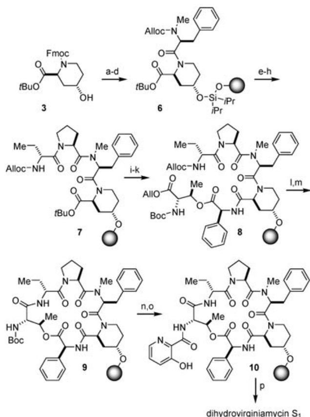
Scheme 3. Solid-phase synthesis of dhVS 1 . a) diisopropyldichlorosilane, imidazole, 30 min; b) hydroxymethyl-polystyrene resin, 48 h; c) 30% piperidine, CH 2 Cl 2 , 30 min; d) Alloc-MePhe-OH, HOAt, DIC, 2,6-lutidine, DMF, 48 h; e) Pd(PPh 3 ) 4 (cat), Bu 3 SnH, 5% AcOH, CH 2 Cl 2 , 3 h; f) Fmoc-Pro-OH, HOAt, DIC, 2,6-lutidine, DMF, 48 h (×3); g) 30% piperidine, CH 2 Cl 2 , 30 min; h) Alloc-D-Abu-OH, HOAt, DIC, 2,6-lutidine, DMF, 24 h; i) TMS-OTf, 2,6-lutidine, CH 2 Cl 2 , 5 h; j) MeOH, 20 min; k) 5 , HOAt, DIC, 2,6-lutidine, DMF, 6 h; l) [Pd(PPh 3 ) 4 ] (cat) , PhSiH 3 , CH 2 Cl 2 , 5 h; m) PyAOP, 2,6-lutidine, CH 2 Cl 2 , 48 h; n) TMS-OTf, 2,6-lutidine, CH 2 Cl 2 , 2 h, 23 °C, then 20 min, 4 °C; o) 3-hydroxypicolinic acid, PyAOP, 2,6-lutidine, THF, 4 h, 4 °C, then 10 h, 23 °C; p) HF/pyridine, THF, 1 h, 15% overall. HOAt = 1-hydroxy-7-azabenzotriazole, DMF = N,N -dimethylformamide, Abu = 2-aminobutyric acid, PyAOP = 7-aza-benzotriazole-1-yloxytris(pyrrolidinophosphonium) hexafluorophosphate.
