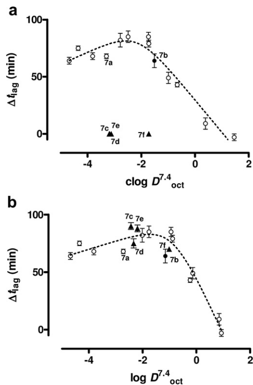
Fig. 1. a) Relationship between antioxidant activity (expressed as \Delta t_{lag} ) and calculated lipophilicity ( \log D^{7.4}_{oct} ) obtained for carnosine amide derivatives (○) [21] and for new compound 7b (●). Calculated \log D^{7.4}_{oct} for designed NO-donor analogues 7c–f (▲) is also reported. b) Relationship between antioxidant activity (expressed as \Delta t_{lag} ) and measured lipophilicity ( \log D^{7.4}_{oct} ) obtained for all carnosine amide derivatives: (○) compounds described in [21], (●) new reference compound 7b, (▲) NO-donor carnosine analogues 7c–f.
