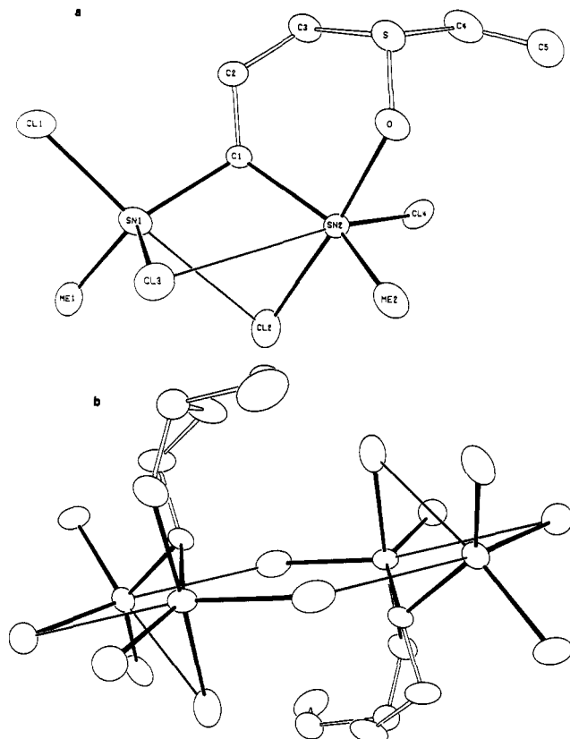
Figure 2. (a) Schematic representation of binuclear unit of 3,3-bis(dichloromethylstannyl)propyl ethyl sulfoxide [(\text{Cl}_2\text{MeSn})_2\text{CHCH}_2\text{CH}_2\text{S}(\text{O})\text{Et}] , 2. (b) Schematic representation of the loosely associated bimolecular unit, resulting from the \text{Sn}(1)\cdots\text{Cl}(4)' and \text{Sn}(1')\cdots\text{Cl}(4) interactions.
