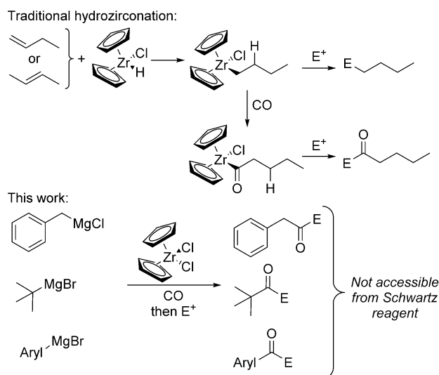
Scheme 1. Synthesis and reactivity of acyl zirconocenes. \text{E}^+ = electrophile.
