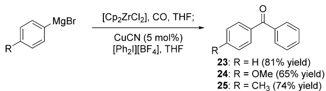
Scheme 4. Carbonylative coupling of aryl Grignard reagents with iodonium salts.
