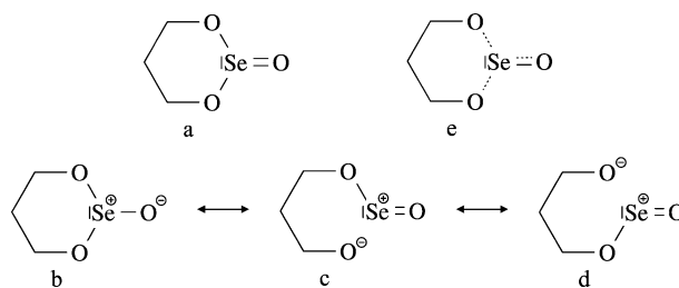
Figure 16. Resonance structures for 8 .
