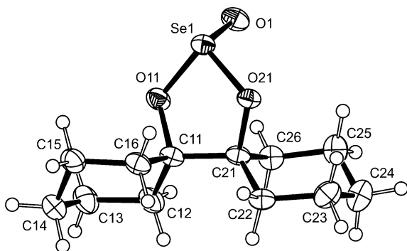
Figure 5. One of the two symmetrically independent molecules of (BhxdH 2 )SeO in crystals of 7 (50% probability ellipsoids, hydrogen atoms with arbitrary radii). Interatomic distances [Å] and angles [°] (with standard deviations of the last digit in parentheses): Se1–O1 1.6177(15), Se1–O11 1.7838(16), Se1–O21 1.7768(16); O1–Se1–O11 101.93(8), O1–Se1–O21 106.82(8), O11–Se1–O21 90.19(7); O11–C11–C21–O21 45.5(2).
