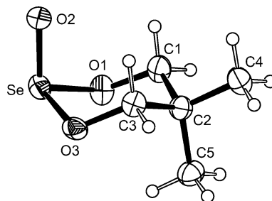
Figure 7. Structure of (DmpdH 2 )SeO in crystals of 9 (40% probability ellipsoids, hydrogen atoms with arbitrary radii). Interatomic distances [Å] and angles [°] (with standard deviations of the last digit in parentheses): Se–O2 1.611(3), Se–O1 1.768(4), Se–O3 1.775(4); O1–Se–O2 104.5(2), O2–Se–O3 104.13(18), O1–Se–O3 95.96(16).
