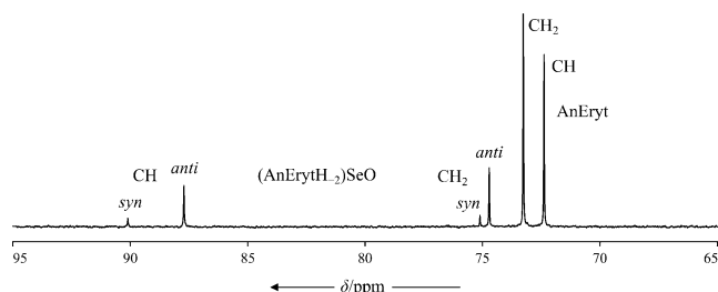
Figure 1. ^{13}\text{C} NMR spectrum of a stoichiometric mixture of 1,4-anhydroerythritol (AnEryt) and \text{SeO}_2 in methanol.
