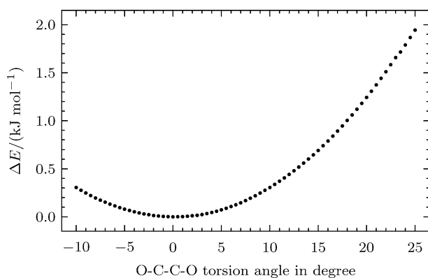
Figure 12. Total energy [B3LYP/6-31+G(2d,p), with an ultra-fine integration grid and very tight convergence criteria] of anti -( cis -1,2-CpdtH 2 )SeO ( 3 ) as a function of the O–C–C–O torsion angle.
