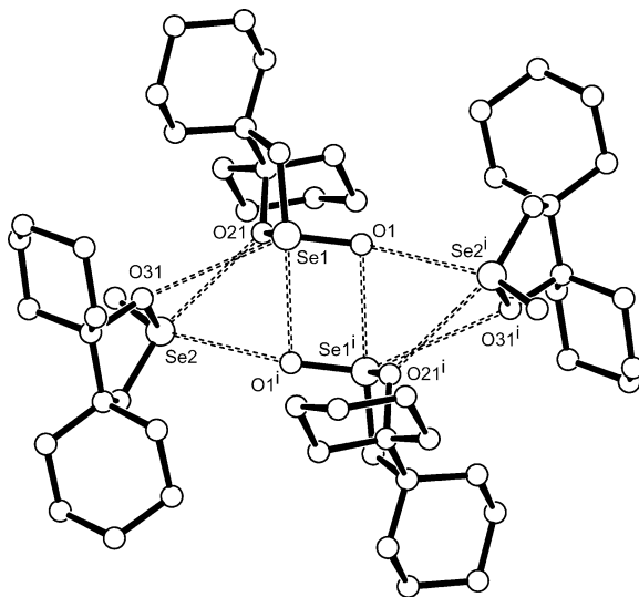
Figure 6. Isolated tetramers in the crystal structure of (BhxdH 2 )SeO ( 7 ) (atoms with arbitrary radii, hydrogen atoms are omitted for clarity). Interatomic distances [Å] (with standard deviations of the last digit in parentheses): Se1–O1 i 2.8113(18), Se1–O31 3.4322(16), O1–Se2 i 3.2417(17), O21–Se2 3.0833(16), Se1–Se1 i 3.4443(3). Symmetry codes: i 1 – x , – y , 1 – z .
