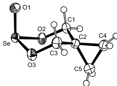
Figure 8. Structure of (BhmrH 2 )SeO in crystals of 10 (50% probability ellipsoids, hydrogen atoms with arbitrary radii). Interatomic distances [Å] and angles [°] (with standard deviations of the last digit in parentheses): Se–O1 1.614(2), Se–O2 1.788(2), Se–O3 1.799(2); O1–Se–O2 104.66(11), O1–Se–O3 102.48(11), O2–Se–O3 95.30(10).
