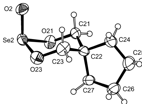
Figure 9. One of the two symmetrically independent molecules of (BhmtH 2 )SeO in crystals of 11 (40% probability ellipsoids, hydrogen atoms with arbitrary radii). Interatomic distances [Å] and angles [°] (with standard deviations of the last digit in parentheses): Se2–O2 1.602(4), Se2–O21 1.758(4), Se2–O23 1.769(4); O2–Se2–O21 105.4(2), O2–Se2–O23 104.85(19), O12–Se2–O23 95.75(16).
