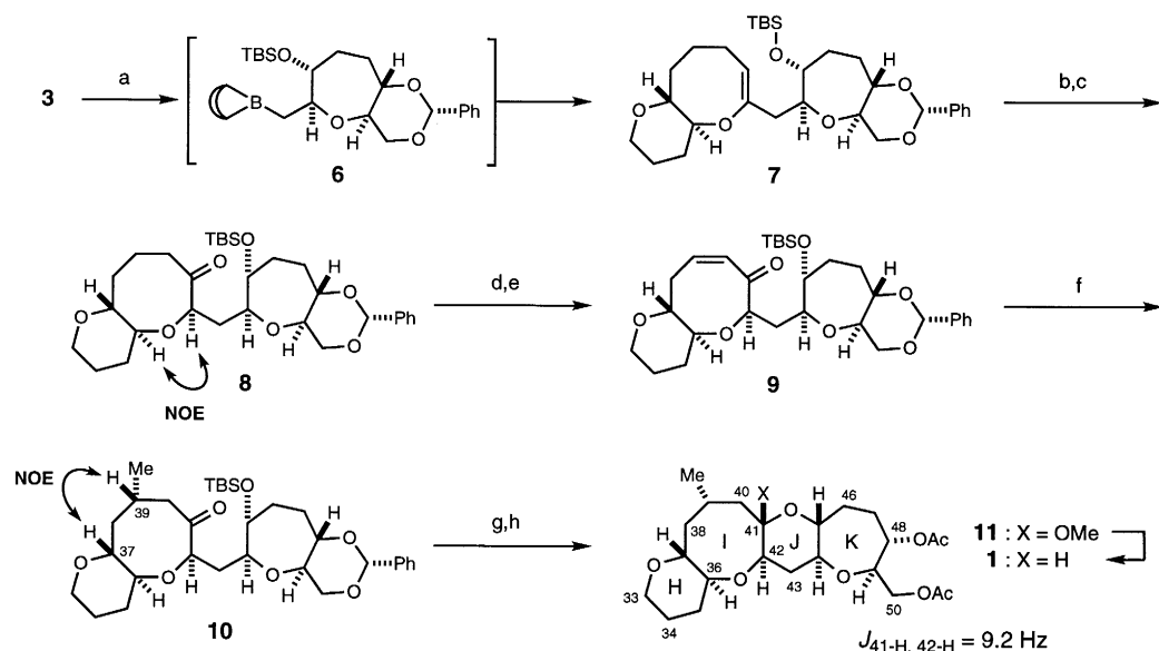
Scheme 3. Reagents and conditions: (a) 9-BBN, THF, rt, then 1 M NaHCO 3 , 2 , Pd(PPh 3 ) 4 , DMF, 50°C, 86%; (b) hexylborane, THF, 0°C, H 2 O 2 , NaOH, rt, 75%; (c) TPAP, NMO, 4 Å MS, CH 2 Cl 2 , rt, quant.; (d) LiHMDS, TMSCl, Et 3 N, THF, -78°C; (e) Pd(OAc) 2 , CH 3 CN, 60°C, 77% (two steps); (f) Me 2 CuLi, Et 2 O, -20°C, 71%; (g) p -TsOH, MeOH, rt, 98%; (h) Ac 2 O, DMAP, CH 2 Cl 2 , 0°C, 97%; (i) Et 3 SiH-BF 3 ·OEt 2 , CH 2 Cl 2 -CH 3 CN (1:1), 0°C, 90%
