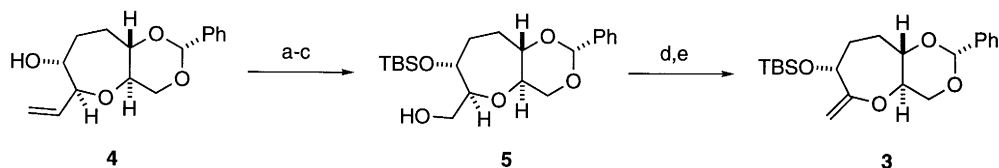
Scheme 2. Reagents and conditions: (a) TBSCl, imidazole, DMF, rt, 73%; (b) OsO 4 , NMO, acetone:H 2 O (4:1), rt, then NaIO 4 , rt; (c) NaBH 4 , MeOH, 0°C, 95% (two steps); (d) I 2 , Ph 3 P, imidazole, benzene, rt; (e) KO t -Bu, THF, 0°C, 96% (two steps)
