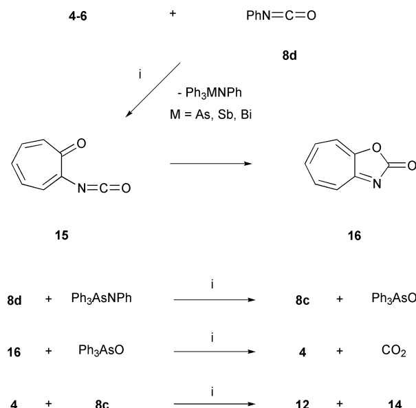
Scheme 4 Conditions: i , heat.
