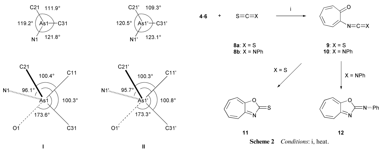
Fig. 3 Bond angles around nearly the trigonal bipyramidal structure of conformations I and II for 4 .
