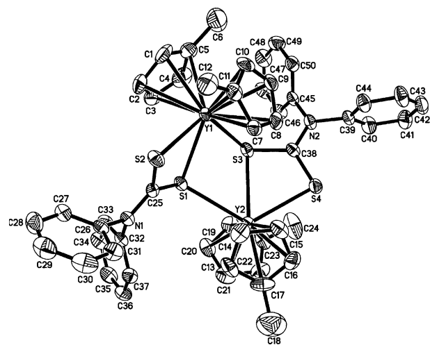
Fig. 8. Molecular structure of [(\text{MeC}_5\text{H}_4)_2\text{Y}(\mu\text{-CS}_2)\text{NPh}_2]_2 .
