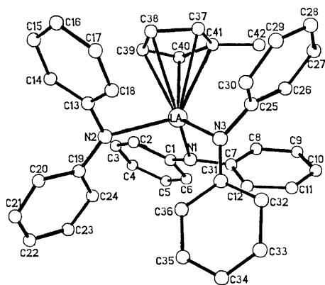
Fig. 1. Molecular structure of [\text{Li}(\text{DME})_3][(\text{MeCp})\text{La}(\text{NPh}_2)_3] .
