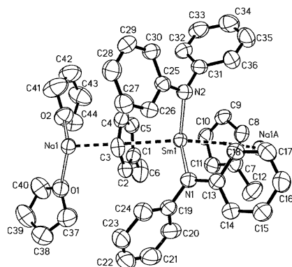
Fig. 2. Molecular structure of [\text{Na}(\text{THF})_2(\mu\text{-}\eta^5\text{:}\eta^5\text{-CH}_3\text{C}_5\text{H}_4)_2\text{Sm}(\text{NPh}_2)_2]_n .
