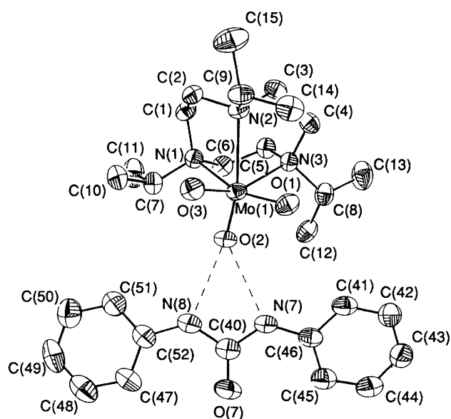
Fig. 8 Structure of one crystallographically independent unit [MoLO 3 ] 3 ·(PhNH) 2 CO in crystals of complex 9
