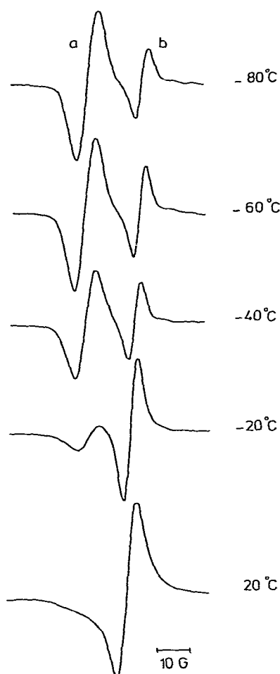
Fig. 1. EPR spectrum of \text{Cp}_2\text{TiC}_2\text{H}_5 (a; g = 1.987 ) in toluene on warming to 20^\circ\text{C} : thermal decomposition (b; decomposition product g = 1.977 ); DPPH external reference.
