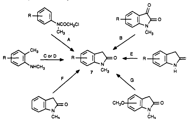
Scheme 2. Syntheses of Substituted 1,3-Dihydro-1-methyl-2 H -indol-2-ones a
