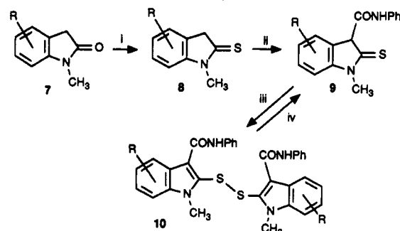
Scheme 1. Synthesis of 1-Methyl- N -phenyl-1 H -indole-3-carboxamides and 2,2'-Dithiobis(1-methyl- N -phenyl-1 H -indole-3-carboxamides) a
