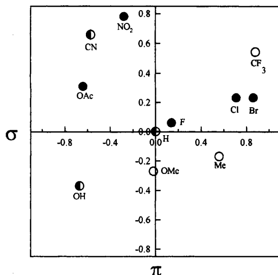
Figure 1. Relationship between substituent electronic and lipophilic properties and EGFR tyrosine kinase inhibition for 5-substituted 2,2'-dithiobis(1-methyl-N-phenyl-1H-indole-3-carboxamides): (●) IC_{50} < 10 \mu M , (◐) IC_{50} 10\text{--}100 \mu M , (○) IC_{50} > 100 \mu M .
