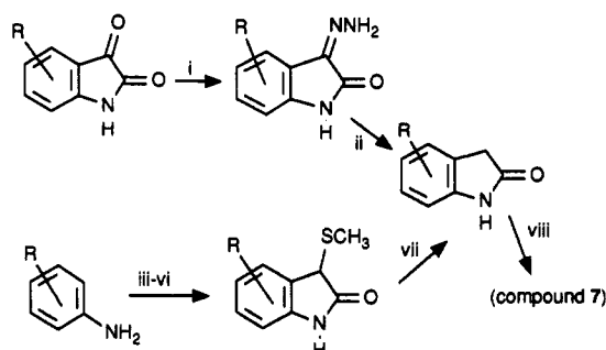
Scheme 3. Synthesis of Substituted 1,3-Dihydro-2 H -indol-2-ones a
