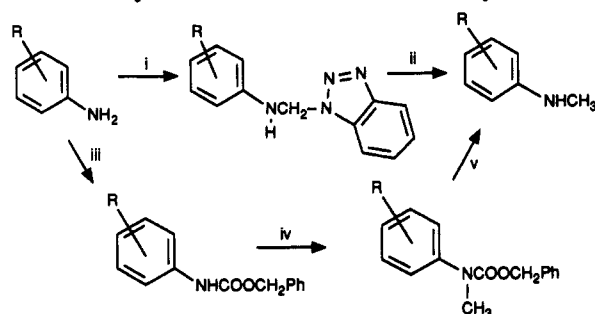
Scheme 4. Synthesis of Substituted N -Methylanilines a
