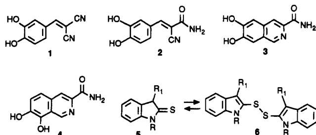
Scheme 1. Synthesis of 1-Methyl- N -phenyl-1 H -indole-3-carboxamides and 2,2'-Dithiobis(1-methyl- N -phenyl-1 H -indole-3-carboxamides) a
