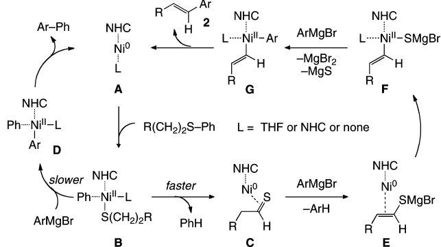
Scheme 2. A Plausible Mechanism
