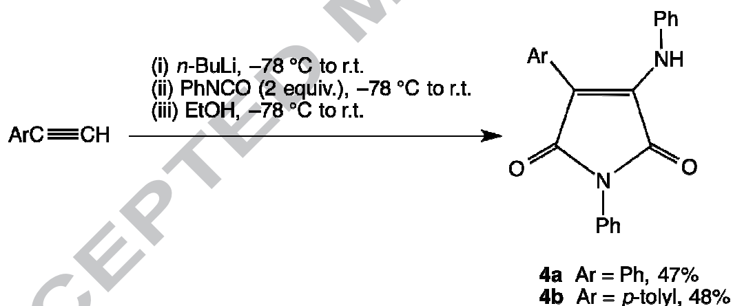
Scheme 1. Formation of the aminomaleimides.
