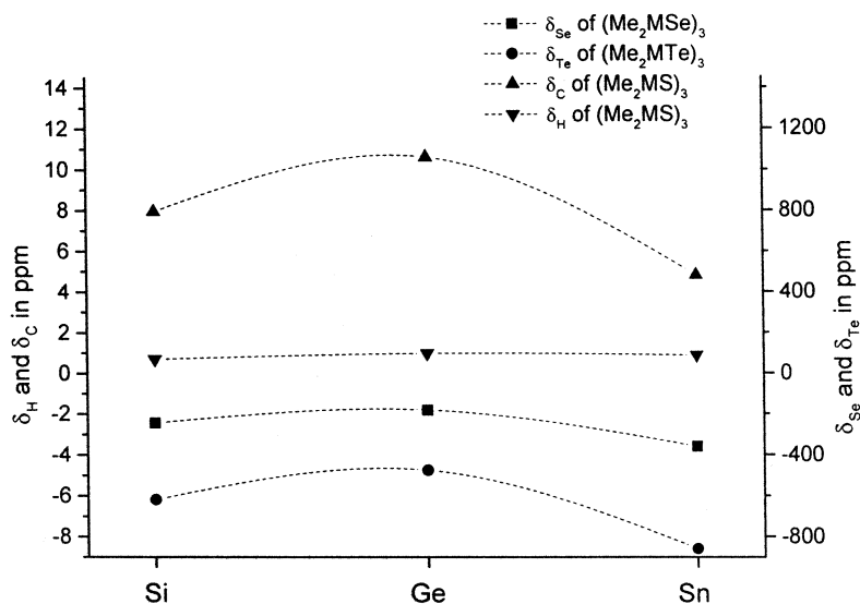
Fig. 1. NMR chemical shifts in six-membered rings (\text{Me}_2\text{ME})_3 ( \text{M} = \text{Si}, \text{Ge}, \text{Sn} ; \text{E} = \text{S}, \text{Se}, \text{Te} ).
