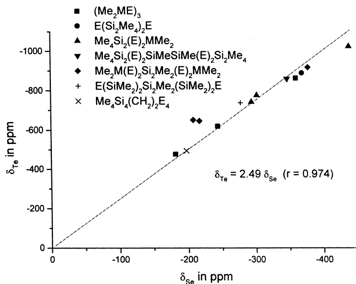
Fig. 2. Correlation of \delta_{\text{Se}} and \delta_{\text{Te}} in different kinds of silselenanes and siltelluranes and related germanium and tin derivatives ( \text{M} = \text{Si}, \text{Ge}, \text{Sn} ; \text{E} = \text{Se}, \text{Te} ) reported here and in Refs. [3,4] ( r = regression coefficient).
