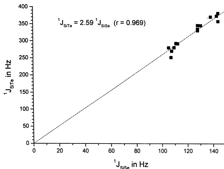
Fig. 3. Correlation of ^1J_{\text{SiSe}} and ^1J_{\text{SiTe}} in different kinds of silselenanes and siltelluranes reported here and in Refs. [3,4] (same compounds as in Fig. 2).
