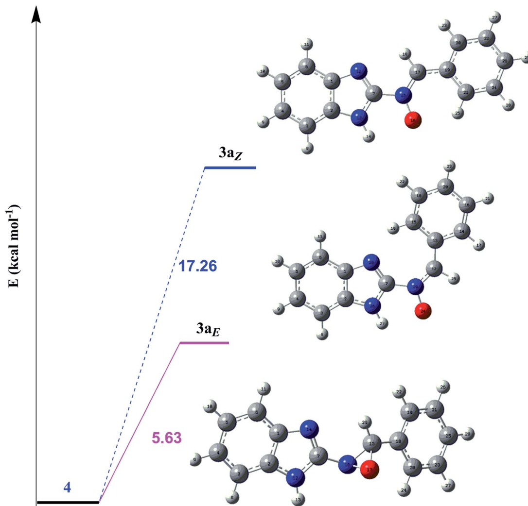
Fig. 3 The optimized structures and relative energy comparison of the nitrone ( 3a_z , 3a_E ) and oxaziridine ( 4 ) molecules.
