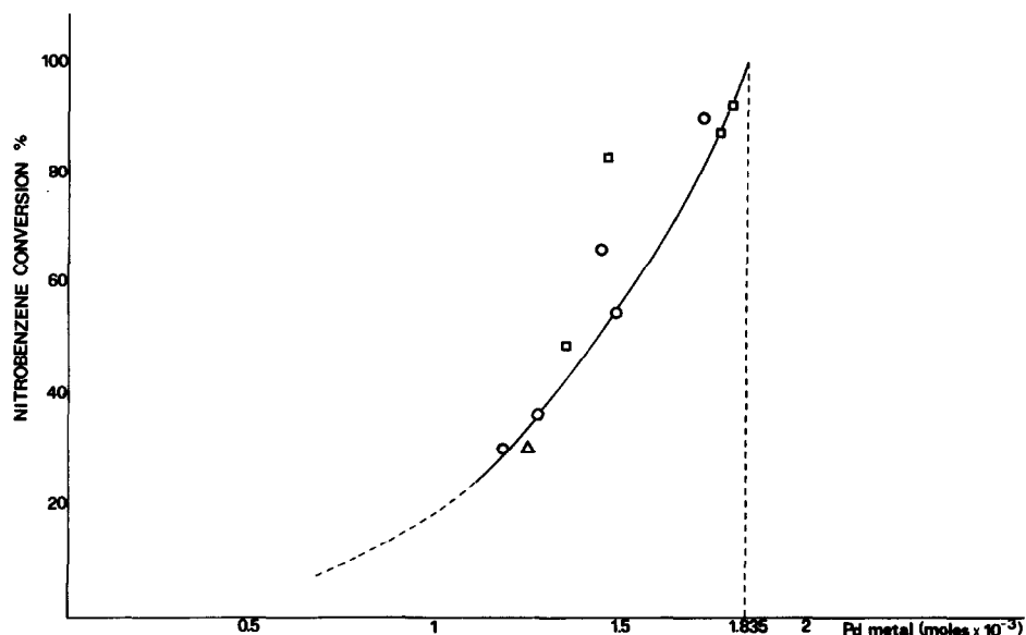
Fig. 10. Reduction of [\text{Pd}(\text{isoquinoline})_2\text{Cl}_2] to metal as a function of initial nitrobenzene conversion. Conditions are: [\text{Pd}(\text{isoquinoline})_2\text{Cl}_2] 1.835 \times 10^{-3} mol, \text{Fe}_2(\text{MoO}_4)_3 1.2 g, solvent 1,2-dichlorobenzene (40 ml), temperature 160^\circ\text{C} , 200 atm of CO pressure. □, Initial concentration of nitrobenzene 0.43 \text{ mol l}^{-1} ; ○, initial concentration of nitrobenzene 1.08 \text{ mol l}^{-1} ; Δ, initial concentration of nitrobenzene 2.16 \text{ mol l}^{-1} .
