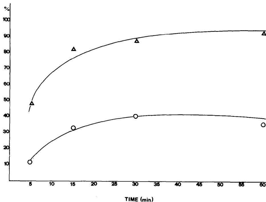
Fig. 4. Conversion of nitrobenzene at 160°C and under 200 atm of CO; [\text{Pd}(\text{isoquinoline})_2\text{Cl}_2] 0.8 g, \text{Fe}_2(\text{MoO}_4)_3 1.2 g, nitrobenzene 2.4 g, solvent 1,2-dichlorobenzene (40 ml). All reagents are added at room temperature, the time to reach 160°C is about 30 min. Δ, Nitrobenzene conversion; ○, phenylisocyanate yields.
