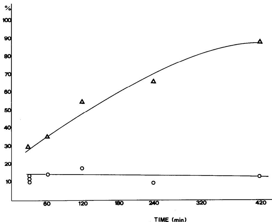
Fig. 3. Conversion of nitrobenzene at 160 °C and under 200 atm of CO; [Pd(isoquinoline)_2Cl_2] 0.8 g, Fe_2(MoO_4)_3 1.2 g, nitrobenzene 6 g, solvent 1,2-dichlorobenzene (40 ml). All reagents are added at room temperature, the time to reach 160 °C is about 30 min. Δ, Nitrobenzene conversion; ○, phenylisocyanate yields.
