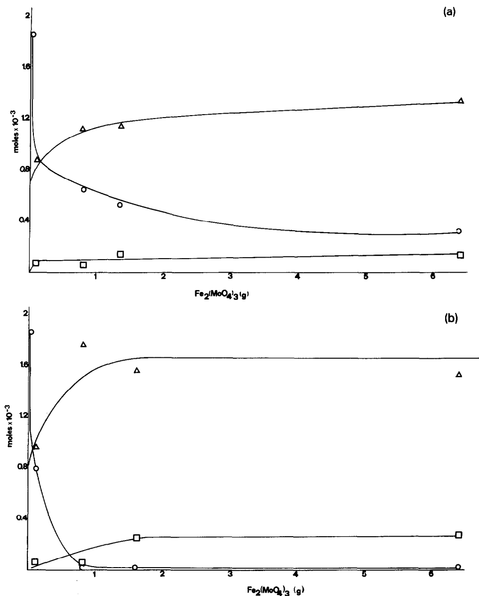
Fig. 8a. Influence of the amount of cocatalyst added on the decomposition of the initial complex [Pd(isoquinoline) 2 Cl 2 ]; Δ, metallic palladium; □, soluble form of palladium; ○, [Pd(isoquinoline) 2 Cl 2 ]. Conditions are: reaction time 30 min, temperature 160°C, 200 atmospheres of CO pressure, [Pd(isoquinoline) 2 Cl 2 ] 1.835 \times 10^{-3} mol, solvent 1,2-dichlorobenzene (40 ml). Initial concentration of nitrobenzene 1.08 mol l -1 , final concentration of nitrobenzene 0.54 mol l -1 .
