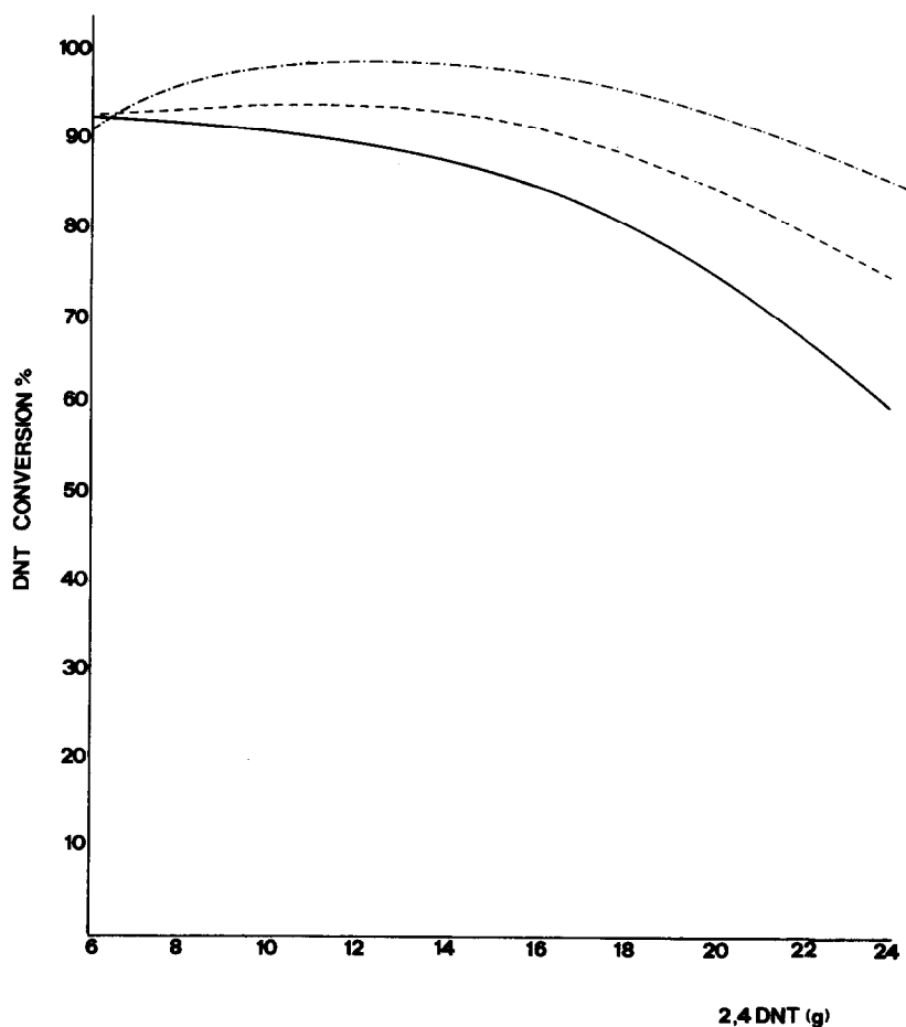
Fig. 12. Conversion of 2,4-DNT as a function of its initial total amount; reaction conditions are those standard of Table 3. — · — · — ·: with 1 g of [\text{Pd}(\text{isoquinoline})_2\text{Cl}_2] and 180 min for the second step of reaction; - - - - -: with 1 g of [\text{Pd}(\text{isoquinoline})_2\text{Cl}_2] and 120 min for the second step of reaction; —: with 1 g of [\text{Pd}(\text{isoquinoline})_2\text{Cl}_2] and 40 min for the second step of reaction.
