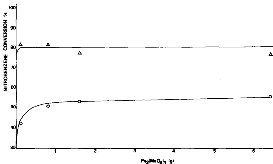
Fig. 9. Influence of the amount of cocatalyst on the conversion of nitrobenzene. Conditions are: reaction time 30 min, temperature 160^\circ\text{C} , 200 atm of CO pressure, [\text{Pd}(\text{isoquinoline})_2\text{Cl}_2] 1.835 \times 10^{-3} mol, solvent 1,2-dichlorobenzene (40 ml). ○, Initial concentration of nitrobenzene 1.08 \text{ mol l}^{-1} ; Δ, initial concentration of nitrobenzene 0.43 \text{ mol l}^{-1} .
