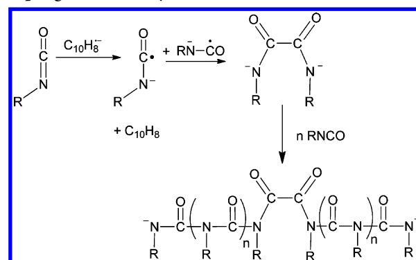
Scheme 1. Formation of Polyisocyanate Initiated by the Coupling of Two Isocyanate Anion Radicals
