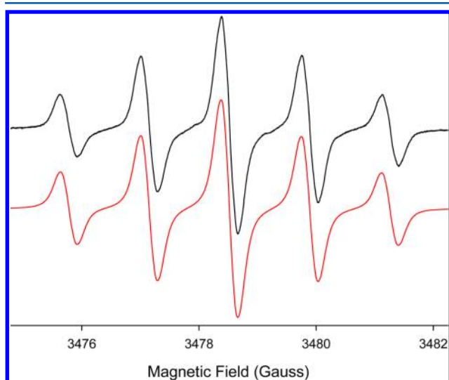
Figure 5. (Upper) EPR spectrum recorded at 295 K after a THF solution containing phenyl isocyanate was exposed to K metal under vacuum. (Lower) Computer-generated EPR spectrum using a_N of 1.37 G (2 Ns) and a_H of 0.080 G (6 Hs) with \Delta w_{pp} = 0.14 G.
