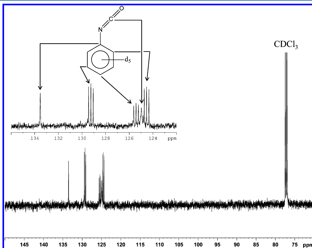
Figure 11. 125 MHz ^{13}\text{C}\{^1\text{H}\} NMR spectrum of synthesized \text{Ph}(^2\text{H}_5)\text{NCO} in \text{CDCl}_3 . Note the carbon resonances that are split into a triplet by the deuterium ( I = 1 ) attached.
