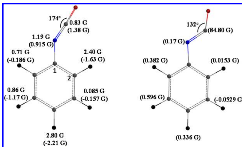
Figure 3. B3LYP/6-311++G**-predicted geometries for two structures of 1 •− . The left structure was obtained by locking the NCO moiety in the same configuration as that obtained for the B3LYP//6-31G* optimized neutral molecule ( \angle NCO = 174°), while in the other calculation no restrictions were made to the NCO group (right structure). All measured coupling constants are shown with the left structure along with the 6-311++G**/EPR-II-computed Fermi contact coupling constants (in parentheses) for both calculated 1 •− structures. The assignment of the measured a_H 's to each proton was made based on the magnitude of the DFT calculated values.
