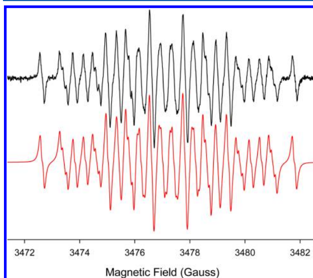
Figure 1. (Upper) X-band EPR spectrum recorded at 295 K after a HMPA solution containing phenyl isocyanate (PhNCO) was exposed to Na metal under vacuum. (Lower) Computer-generated EPR spectrum using a_N of 1.19 G and a_H 's of 2.80, 2.40, 0.860, 0.710, and 0.085 G for five unique protons. The peak-to-peak line width ( \Delta w_{pp} ) is 0.09 G.
