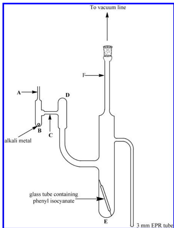
Figure 12. Apparatus used for the generation of the isocyanate and isocyanurate anion radicals in HMPA or THF.
