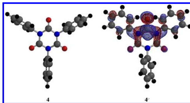
Figure 8. B3LYP/6-31G*-predicted geometries for 4 and 4^{\bullet-} . Structure 4 has D_{3h} symmetry where the plane of the phenyl rings is orthogonal to the planar isocyanurate ring. In the case of 4^{\bullet-} the isocyanurate is no longer flat and the carbonyl with high electron density is slightly pyramidalized. Note that the phenyl rings adjacent to this carbonyl have rotated to become somewhat coplanar with the isocyanurate moiety. Also shown is the shape of the \pi -SOMO surface for 4^{\bullet-} , which supports the experimental result that the electron is localized in one carbonyl.
