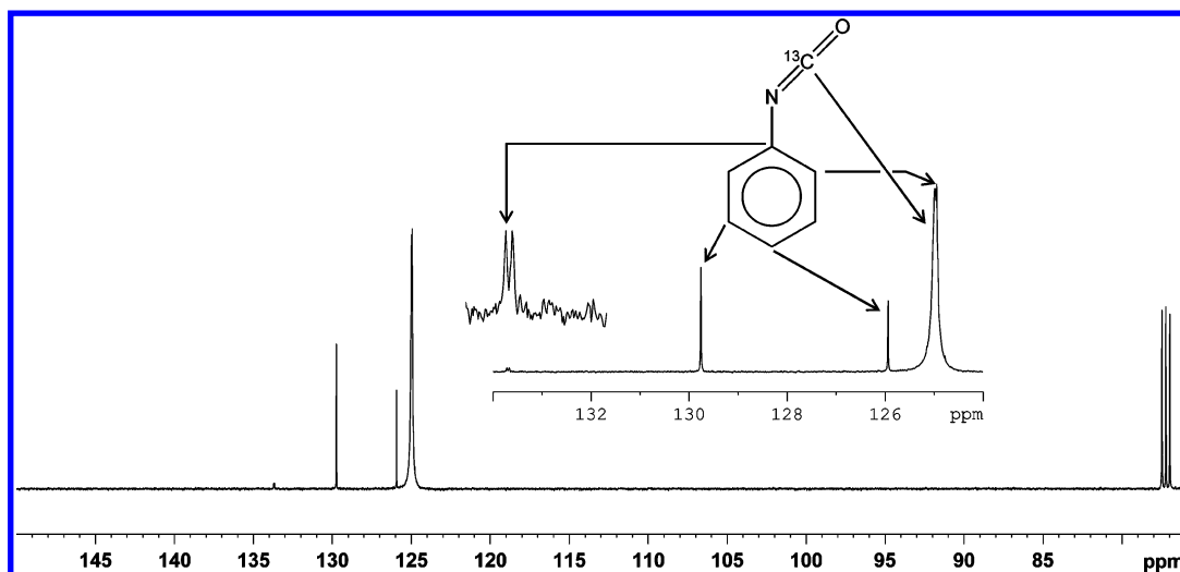
Figure 10. 125 MHz ^{13}\text{C}\{^1\text{H}\} NMR spectrum of \text{PhN}^{13}\text{CO} in \text{CDCl}_3 . Note that the ipso carbon resonance is split by coupling to the isocyanate carbon ( ^2J_{\text{CC}} = 6.3 Hz).
