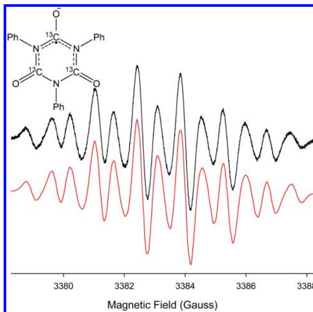
Figure 7. (Upper) EPR spectrum recorded at 295 K after a THF solution containing PhN ^{13}C O was exposed to K metal. (Lower) Computer-generated EPR simulation using a_N = 1.38 G (2 Ns), a_{13C} = 1.52 G ( 1 \times ^{13}C ), a_{13C} = 0.835 G ( 2 \times ^{13}C s) and a_H = 0.10 G (6 Hs), \Delta w_{pp} = 0.15 G.
