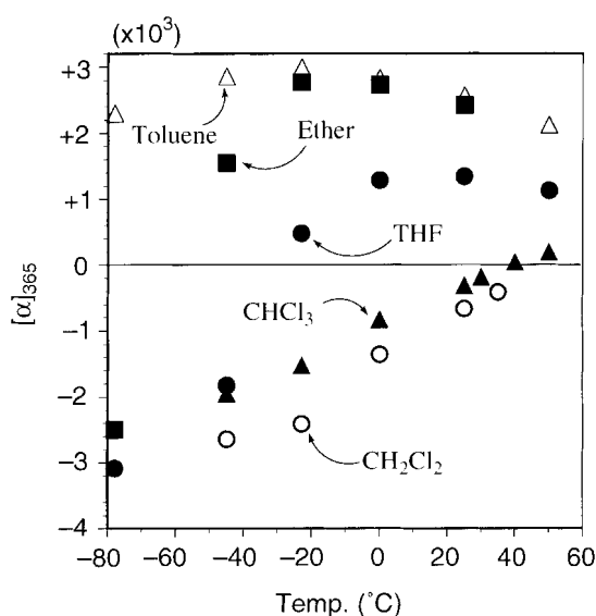
Figure 6. Temperature dependence of specific rotation of poly-2 in toluene ( \Delta ), diethyl ether ( \blacksquare ), THF ( \bullet ), \text{CHCl}_3 ( \blacktriangle ) and \text{CH}_2\text{Cl}_2 ( \circ )
