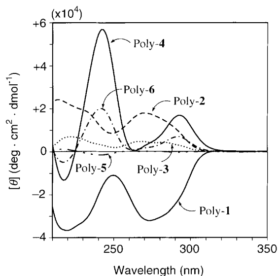
Figure 1. CD spectra of poly(phenyl isocyanate)s bearing an alkoxy group in THF at ambient temperature (ca 23–25°C)
