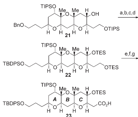
Scheme 4. a) LiDBB, THF, -78 to -40^{\circ}\text{C} (80%); b) TBDPSCl, \text{NEt}_3 , DMAP, \text{CH}_2\text{Cl}_2 , -78^{\circ}\text{C} (95%); c) CSA, \text{CH}_2\text{Cl}_2 , RT (92%); d) TESCl, \text{NEt}_3 , DMAP, \text{CH}_2\text{Cl}_2 (100%); e) AcOH, \text{H}_2\text{O}/\text{MeOH} (97%); f) TPAP, NMO, \text{CH}_2\text{Cl}_2 (97%); g) \text{NaClO}_2 , 2-methyl-2-butene, \text{NaHPO}_4 , \text{H}_2\text{O} , t\text{BuOH} (95%); LiDBB: lithium 4,4'-di- tert -butylbiphenylide, CSA: camphorsulfonic acid.
