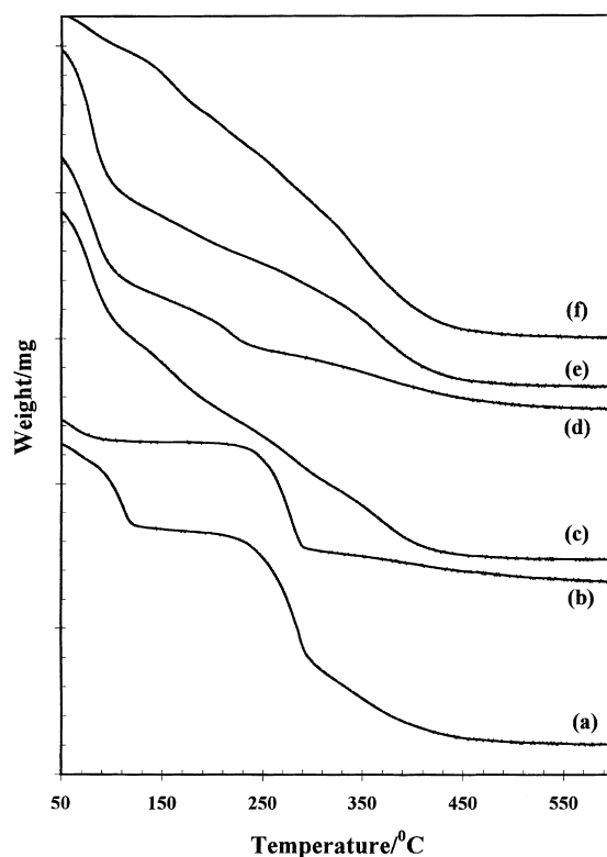
Fig. 3. TGA of alumina gels formed from tri-sec-butoxyaluminum: (a) unmodified at 25°C; (b) unmodified at 90°C; (c) modified with 1 mol of acetic acid and hydrolysed at 90°C; (d) modified with 1 mol of acetic acid and hydrolysed at 25°C; (e) modified with 1 mol of propanoic acid and hydrolysed at 25°C; (f) modified with 1 mol of butanoic acid and hydrolysed at 25°C.
