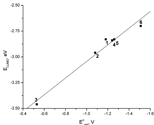
Figure 8. Linear dependence of E_{1/2(red)} and the LUMO energies for complexes 1–6.
