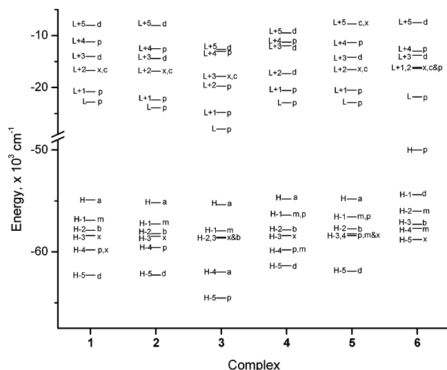
Figure 6. Molecular orbital energy diagram for six occupied (H) and six virtual (L) frontier orbitals of 1–6 in the singlet ground state in ethanol. a = Re d , CNx, b = Re d , CO, c = CO, d = delocalize, m = Re d , p = phen-based ligand, and x = CNx. For example, orbitals H-3 and H-4 of complex 5 are assigned as p,m&x where H-3 is on the phen-based ligand (p) and Re d (m) but H-4 is on the CNx ligand (x).
