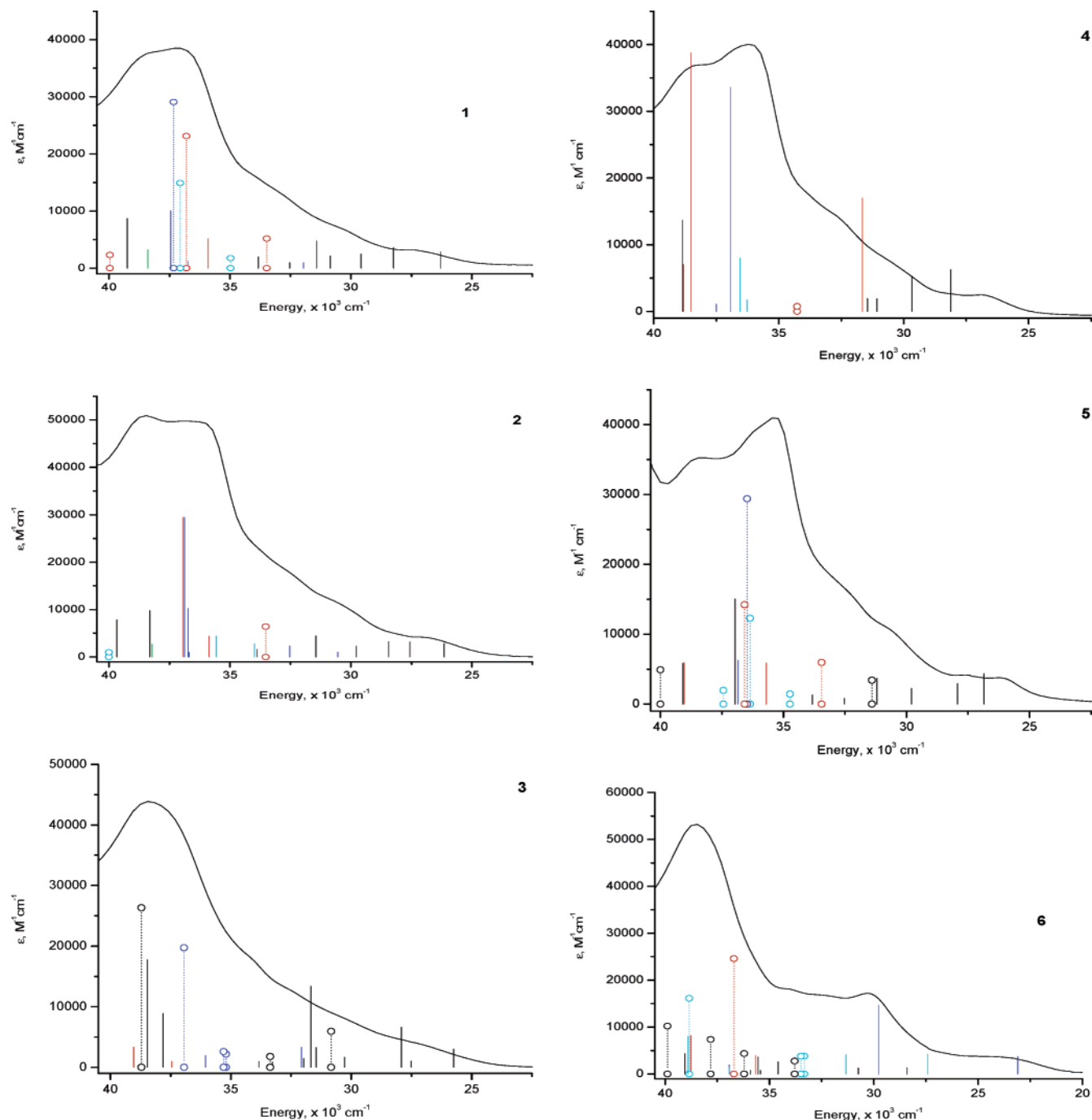
Figure 3. Experimental absorption spectra of 1–6 and calculated singlet excited states. The excited states are shown as vertical bars with height equal to the extinction coefficient. 31a Black = MLCT, green = LLCT, blue = \pi \rightarrow \pi^* , red = MCDCT, cyan = LCDCT (ligand \rightarrow delocalized), and \bigcirc \cdots \bigcirc = mixed excited state.
