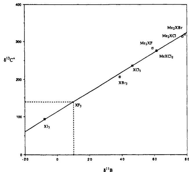
Figure 1. A plot of ^{13}\text{C} NMR chemical shifts of halomethyl cations vs ^{11}\text{B} NMR chemical shifts of isoelectronic isomethanes.
