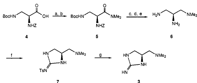
Scheme 1 a
