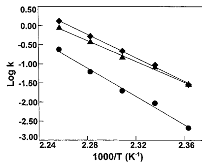
Figure 6. Arrhenius plot for intramolecular cyclization of aspartame for each specific spectrum. Key: ●, 1543 \text{cm}^{-1} ; ◆, 1283 \text{cm}^{-1} ; ▲, 1259 \text{cm}^{-1} .
