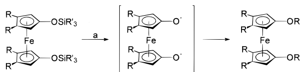
Scheme 5. Synthesis of the 1,1'-Dialkoxyferrocenes a
