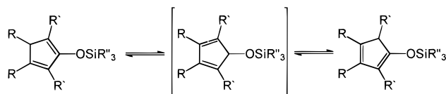
Scheme 4. 1,1'-Disiloxyferrocenes
