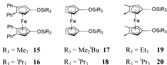
Scheme 4. 1,1'-Disiloxyferrocenes
