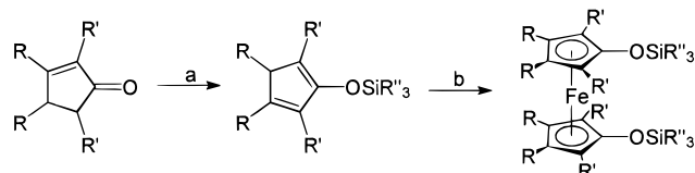
Scheme 1. General Synthesis of the Cyclopentadienyl Silyl Ethers and Ferrocenyl Silyl Ethers a
