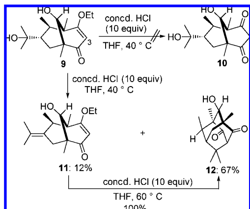
SCHEME 5. Attempted C3-Benzoylation via an Intramolecular Hetero-Michael Reaction
