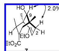
FIGURE 3. 1 H NMR NOE experiment of 7 .
