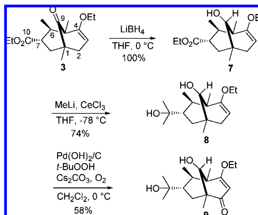
SCHEME 3. Introduction of the C10- gem -Dimethyl Groups and the C2-Carbonyl Group
