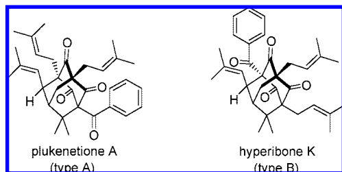
FIGURE 2. PPAPs with an adamantane core.
