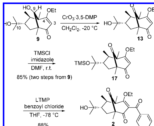
SCHEME 6. C3-Benzoylation via a Vinyl Anion
