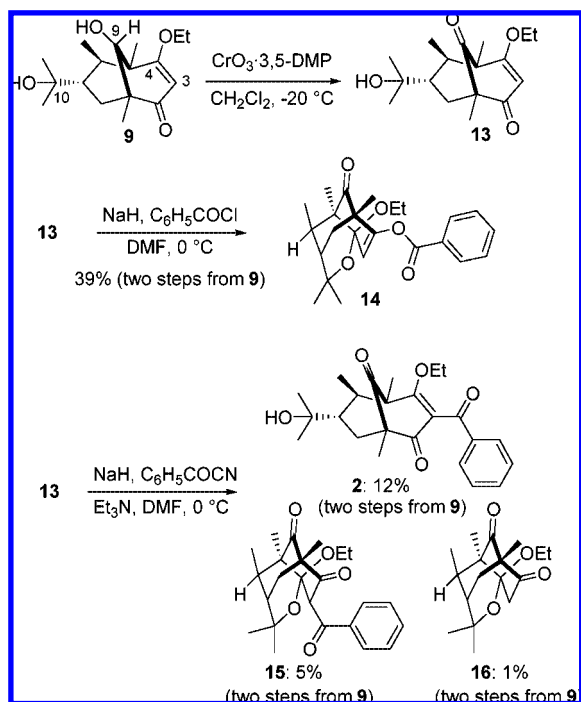
SCHEME 5. Attempted C3-Benzoylation via an Intramolecular Hetero-Michael Reaction
