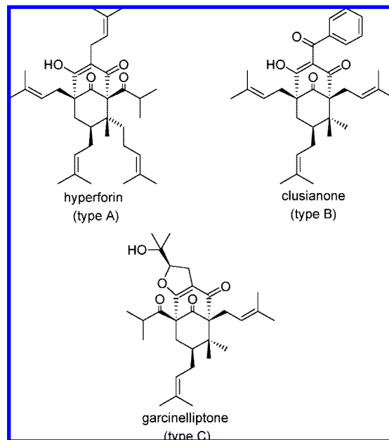
FIGURE 1. PPAPs with a bicyclo[3.3.1]nonane core.
