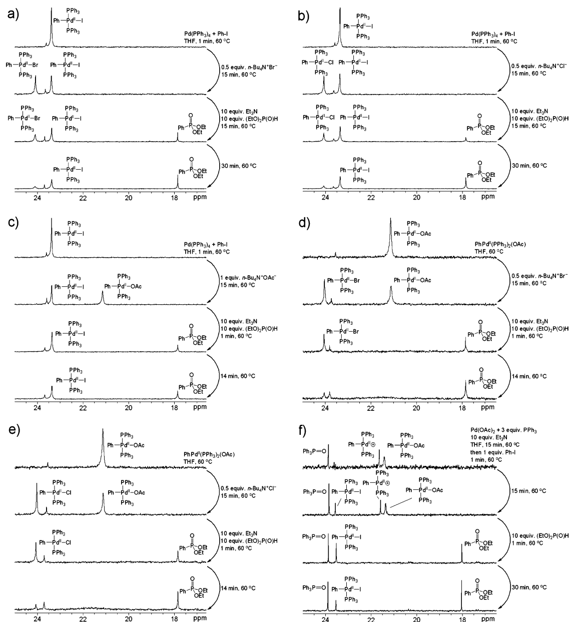
Figure 1. ^{31}\text{P} NMR competition experiments between \text{Pd}(\text{II}) species ligated with different anions in reaction with (\text{EtO})_2\text{P}(\text{O})\text{H} : (a) \text{Br}^- vs \text{I}^- ; (b) \text{Cl}^- vs \text{I}^- ; (c) \text{I}^- vs \text{OAc}^- ; (d) \text{Br}^- vs \text{OAc}^- ; (e) \text{Cl}^- vs \text{OAc}^- ; \text{I}^- vs \text{OAc}^- vs cationic species. Small signal at 23.7 ppm originates from contamination with \text{Ph}_3\text{PO} .
