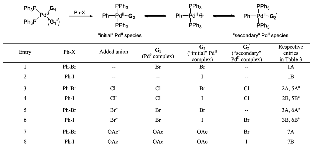
Scheme 6. Formation of Three Pd(II) Species That Might Be Involved in Ligand Exchange Reaction with the H-Phosphonate
