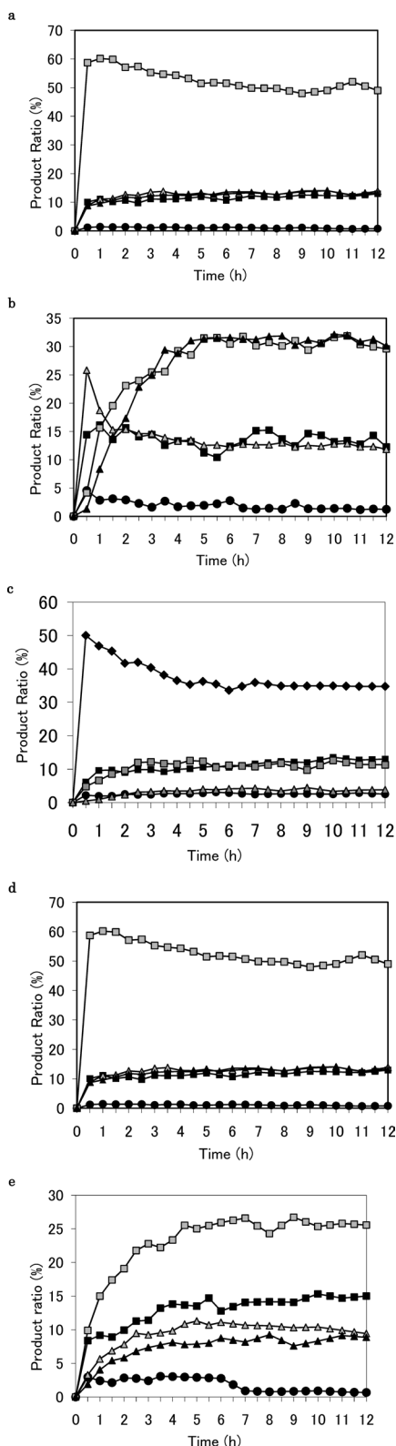
Fig. 2. Product Ratio vs. Reaction Time in the Condensation Reaction of Trimethoxybenzene ( 3 ) with Bis-hydroxymethyl- tert -butylphenol ( 4 ) in the Presence of Yb(OTf) 3 in Refluxing Solvent ( 3 : ●, 5 : ■, 5' : ◆, 6 : □, 7 : △, 8 : ▲)
