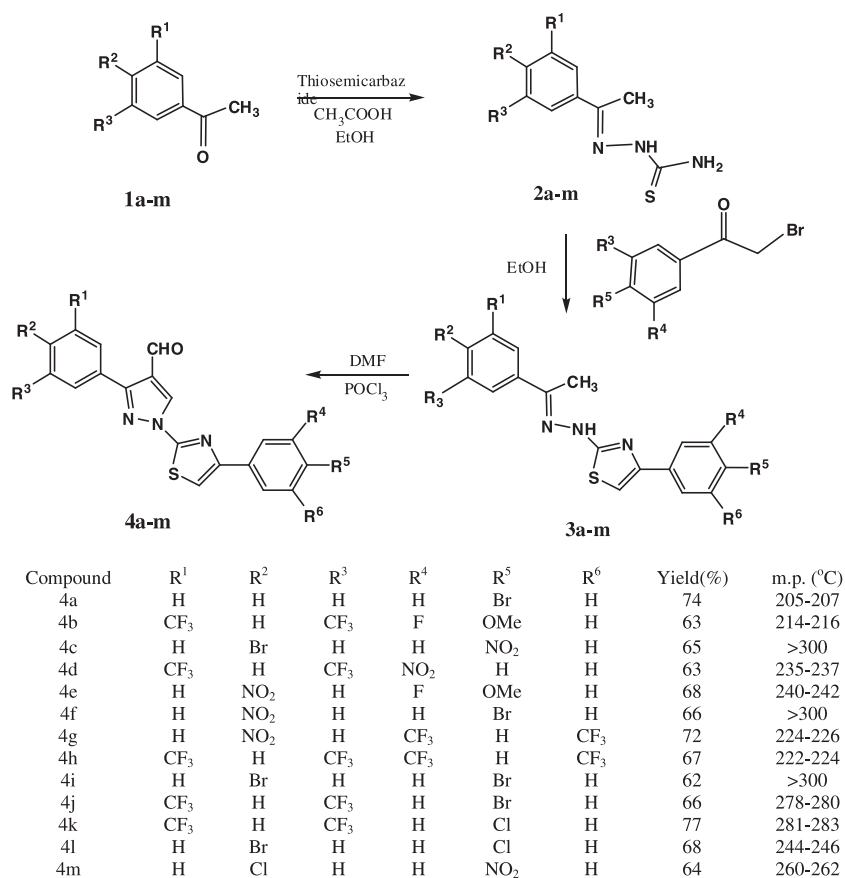
Scheme 1. Synthetic pathway for the formation of compounds 4a-m .
