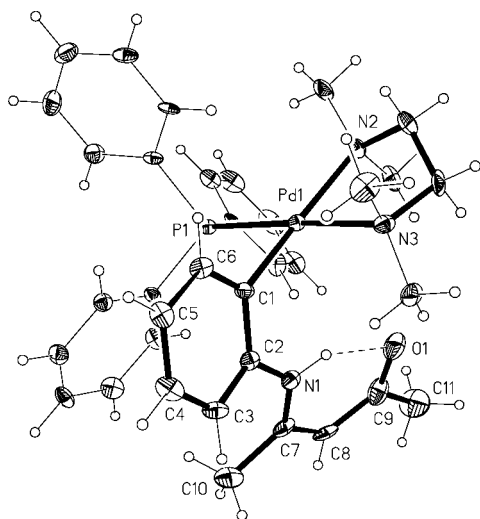
Figure 4. Thermal ellipsoid representation plot (30% probability) of one of the two independent cations of complex 7 . See Supporting Information for bond lengths and angles.
