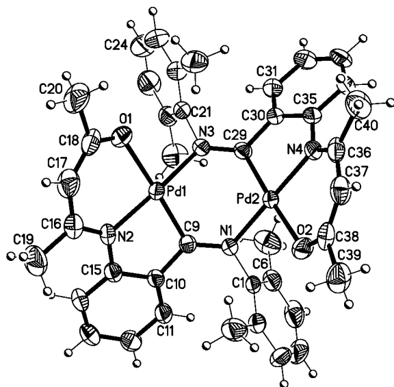
Figure 6. Thermal ellipsoid representation plot (50% probability) of complex 13 . Selected bond lengths (Å) and angles (deg): Pd(1)–C(9) = 1.954(4), Pd(1)–N(2) = 2.002(3), Pd(1)–O(1) = 2.067(3), Pd(1)–N(3) = 2.068(3), Pd(2)–C(29) = 1.931(4), Pd(2)–N(4) = 2.013(3), Pd(2)–N(1) = 2.067(3), Pd(2)–O(2) = 2.072(3), N(1)–C(9) = 1.290(5), N(1)–C(1) = 1.448(5), N(3)–C(29) = 1.294(5), N(3)–C(21) = 1.447(5), N(2)–C(16) = 1.329(5), N(4)–C(36) = 1.326(6), C(16)–C(17) = 1.401(7), C(36)–C(37) = 1.395(7), C(17)–C(18) = 1.386(8), C(37)–C(38) = 1.391(7), O(1)–C(18) = 1.257(6), O(2)–C(38) = 1.270(5), C(9)–Pd(1)–N(2) = 82.82(15), N(2)–Pd(1)–O(1) = 93.20(14), C(9)–Pd(1)–N(3) = 96.99(15), O(1)–Pd(1)–N(3) = 87.85(13), C(29)–Pd(2)–N(4) = 81.44(15), C(29)–Pd(2)–N(1) = 96.36(14), N(4)–Pd(2)–O(2) = 92.58(13), N(1)–Pd(2)–O(2) = 89.99(12), C(15)–N(2)–Pd(1) = 110.1(2), C(35)–N(4)–Pd(2) = 110.6(3), C(10)–C(9)–Pd(1) = 109.8(3), C(30)–C(29)–Pd(2) = 111.1(3), C(18)–O(1)–Pd(1) = 119.2(3), C(38)–O(2)–Pd(2) = 119.0(3), O(1)–C(18)–C(17) = 126.7(4), O(2)–C(38)–C(37) = 127.3(4), N(2)–C(16)–C(17) = 122.3(4), N(4)–C(36)–C(37) = 122.4(4), C(16)–N(2)–Pd(1) = 123.1(3), C(36)–N(4)–Pd(2) = 122.3(3).
