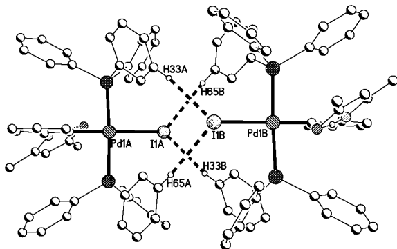
Figure 14. Dimer formation via bifurcated (\text{C-H})_2 \cdots \text{I} interactions in complex 3 . The symmetry operator is 1-x, -y, -z .
