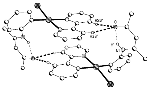
Figure 13. Dimer formation via bifurcated (\text{C-H})_2 \cdots \text{O} interactions in complex 1 . The distance between the stacked ring centroids is 3.7 Å. The symmetry operator is 1/2-x, 1/2-y, 1-z .
