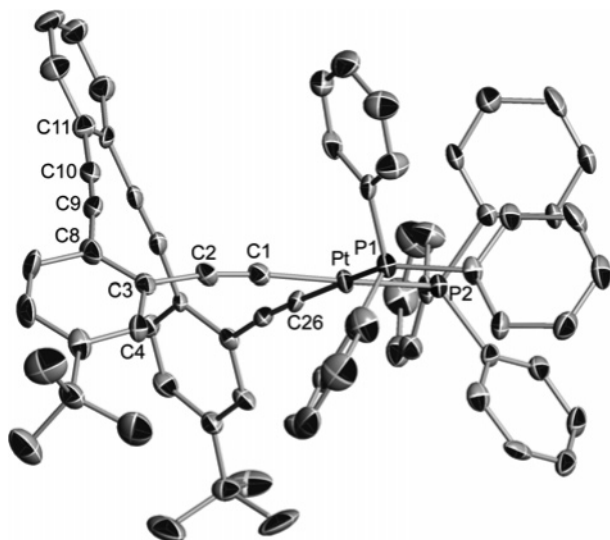
Figure 5. ORTEP of platina-annulene 12 ; ellipsoids drawn at the 50% probability level. Selected bond lengths (Å) and angles (deg): Pt–P1 2.313(18), Pt–C1 1.964(7), C1–C2 1.220(9), C9–C10 1.197(9), P1–Pt–P2 100.2(6), C26–Pt–C1 86.0(3), Pt–C1–C2 175.3(6), C1–C2–C3 174.9(7), C8–C9–C10 174.9(7), C9–C10–C11 171.6(8).
