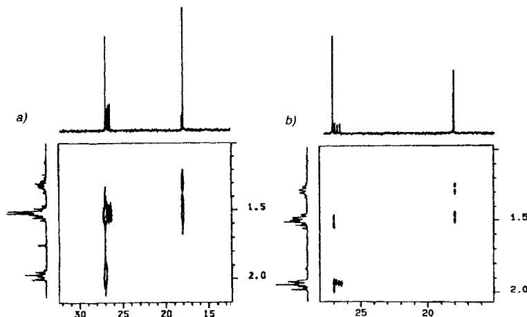
Fig. 9. ^1\text{H} , ^{13}\text{C} -NMR correlation spectra of a) ( \pm )- cis -1,2-epoxy(3- ^2\text{H}_1 )cyclopentane ( 1b ) and b) ( \pm )- trans -1,2-epoxy(3- ^2\text{H} )cyclopentane ( 1a ). The ^2\text{H} -bearing C-atom ( t ) is in the first case correlated with a trans H-atom and in the second case with a cis -H-atom.
