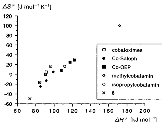
Fig. 10. Correlation of \Delta H^\ddagger and \Delta S^\ddagger for different benzyl- Co III complexes [29] (Saloph = ( N,N' -bis(salicylidene)- o -phenylenediamine, OEP = octaethylporphyrine), methylcobalamin [31], isopropylcobalamin [11], and 6
