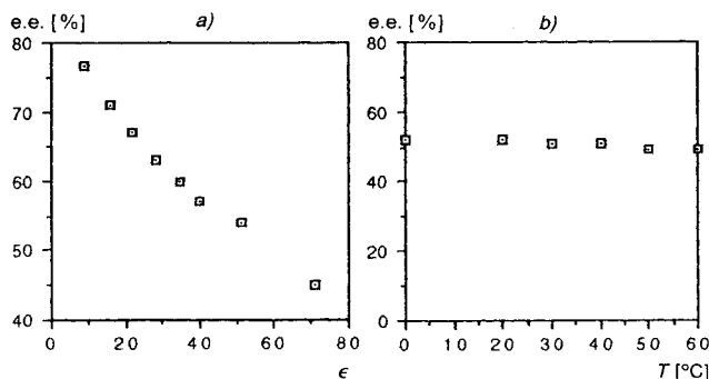
Fig. 2. Enantiomeric excess e.e. of 2 vs. a) the dielectric constant \epsilon and b) the temperature
