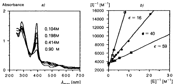
Fig. 4. a) UV/VIS Spectra in the steady state. Mixtures of 2.8 \cdot 10^{-4} M cob(I)alamin, 0.1 M \text{NH}_4\text{Cl} in MeOH ( \epsilon = 28.5 ), Zn powder at different concentrations of 1 (0, 0.104, 0.198, 0.414, and 0.90 M); d = 0.2 cm. b) Reciprocal concentration of 6 versus reciprocal concentration of epoxide 1 in the steady state, at different dielectric constants \epsilon (calc. according to Eqn. 2 and 4).
