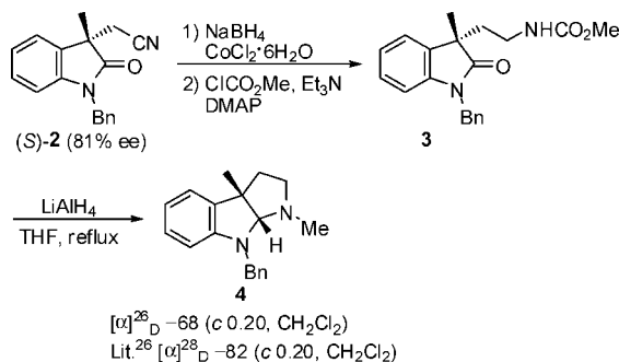
Scheme 1. Determination of Absolute Configuration
