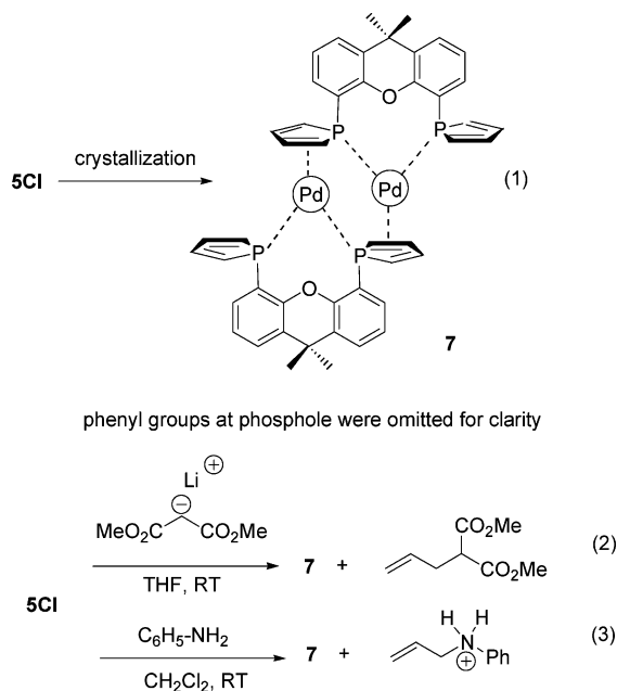
Scheme 6. Three Syntheses of Dimer 7
