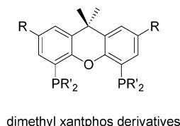
Scheme 1. General Formula of Xantphos Derivatives
