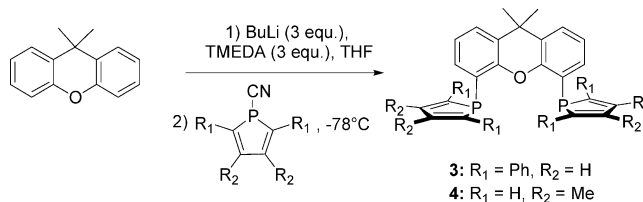
Scheme 3. Synthesis of DPP- and DMP-Xantphos Derivatives 3 and 4
