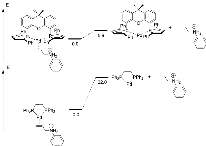
Scheme 9. Activation Energies Needed for the Dissociation of the Phenylallylammmonium Ligand to Produce [Pd(3)] and [Pd(dppe)] Complexes (energies in kcal/mol)
