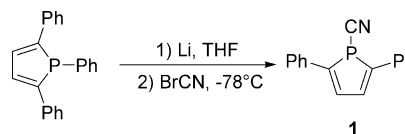
Scheme 3. Synthesis of DPP- and DMP-Xantphos Derivatives 3 and 4
