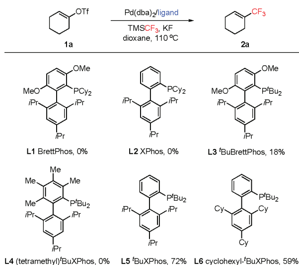
Scheme 1. Ligand Screen for the Trifluoromethylation of Vinyl Triflate 1a a,b
