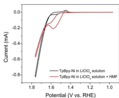
Figure 4 CVs of TpBpy-Ni@FTO in the absence (black line) and in the presence (red line) of 5 mM HMF in 0.1 M LiClO 4 solution (pH = 13).
