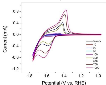
Figure 5 CVs of TpBpy-Ni@FTO in 0.1 M LiClO 4 solution (pH 13) at different scan rates (5–1000 mV s -1 ).
