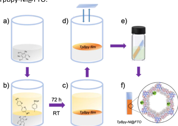
Figure 2 Schematic illustration of the preparation of TpBpy-Ni@FTO.
