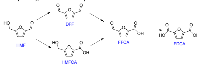
Figure 1 Illustration of two possible reaction pathways of HMF oxidation.
