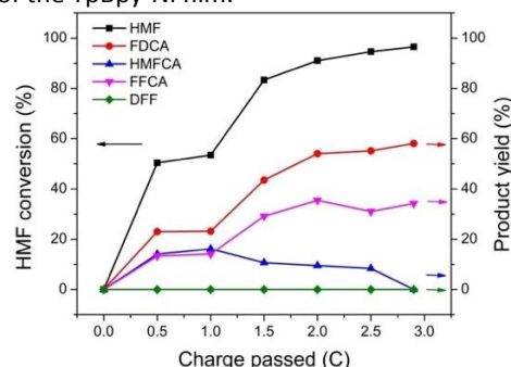
Figure 6 HMF conversion and yields of products after passing 0, 0.5, 1, 1.5, 2, 2.5, 2.9 C. Each data point is average of three tests (see Table S1).
