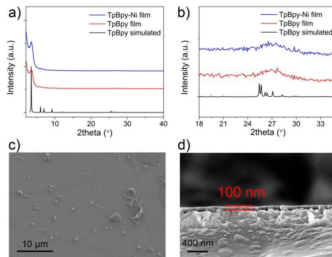
Figure 3 (a) PXRD patterns of simulated TpBpy (black), TpBpy film (red), and TpBpy-Ni film (blue), (b) zoomed-in figure of 18–35° region in (a), (c) top-view SEM image of TpBpy-Ni film, (d) cross-section view SEM image of TpBpy-Ni film.
